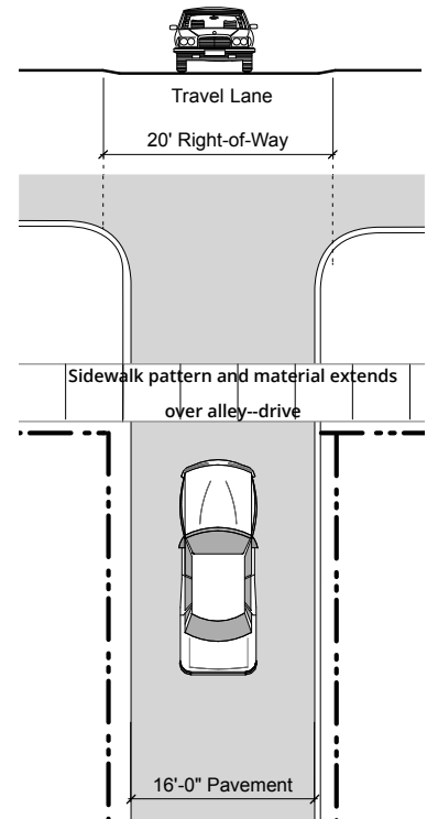
Figure 3.290-C. Typical Alley or Service Drive
